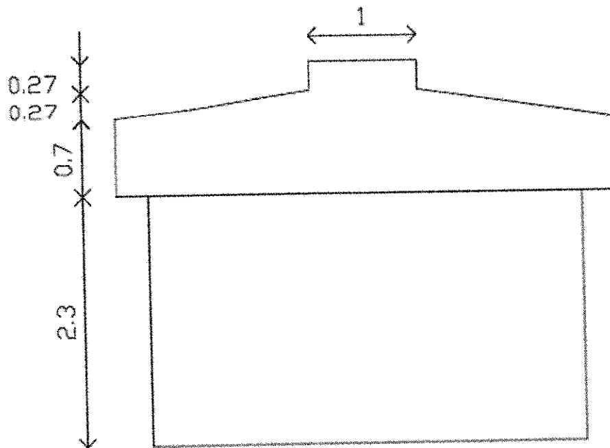
PIGNON
